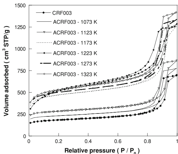
Fig. 10 N 2 adsorption–desorption isotherms at 77 K for ACRF003 carbons at various temperatures
