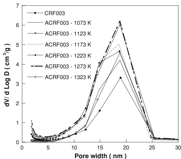
Fig. 11 Pore size distribution of ACRF003 carbons at various temperatures
